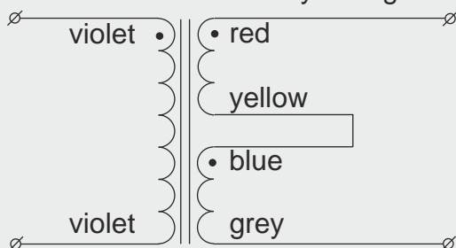
serial operation to double the secondary voltage
