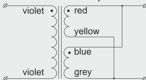
parallel operation to double the secondary current
